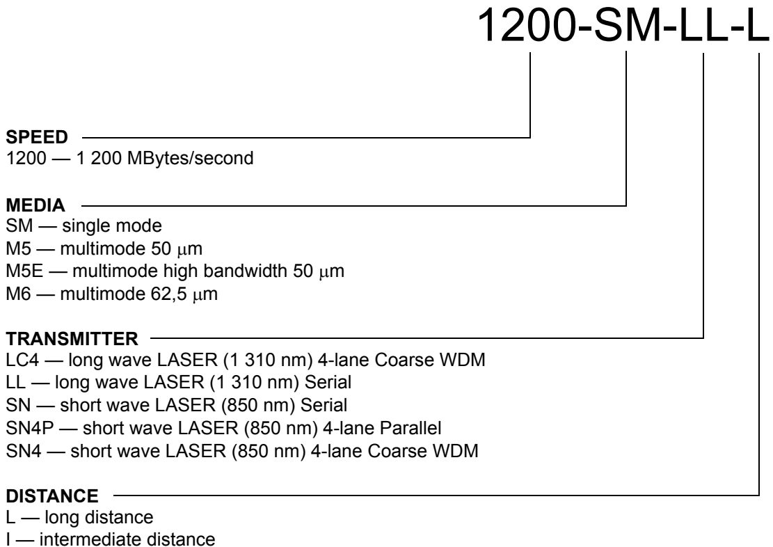
Figure 4 – 10GFC physical variant nomenclature
