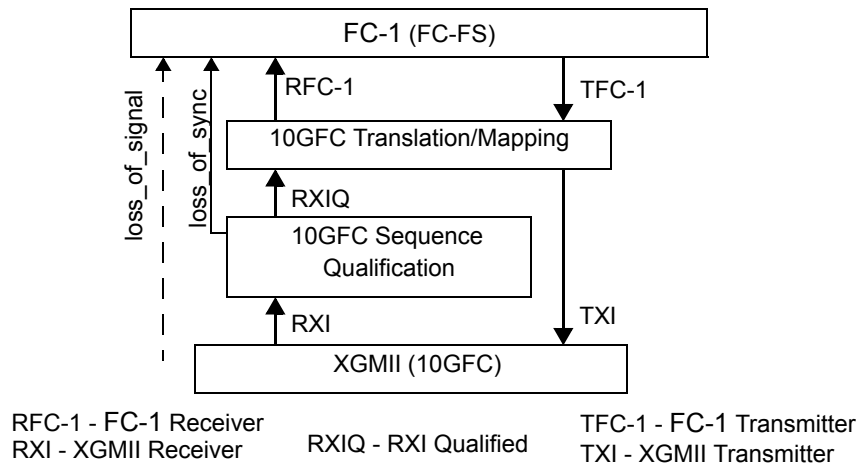
Figure 12 – FC-1/10GFC/XGMII Interaction
