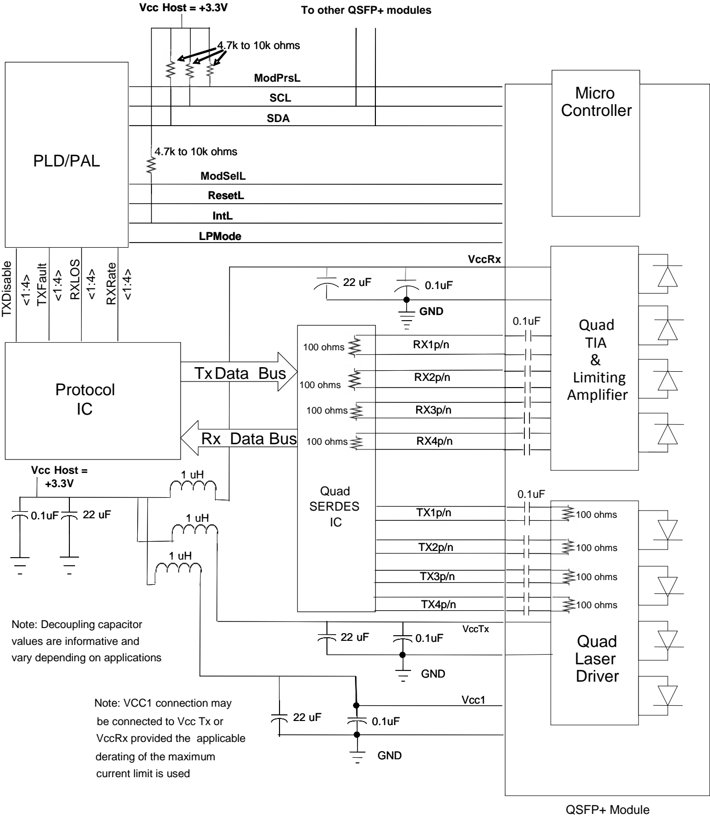
3 4 5 6 Figure 3a: Example QSFP+ Host Board Schematic for optical modules
