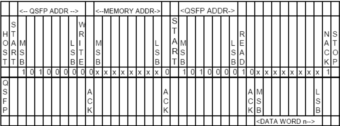
Figure 25 — QSFP+ Random Read
