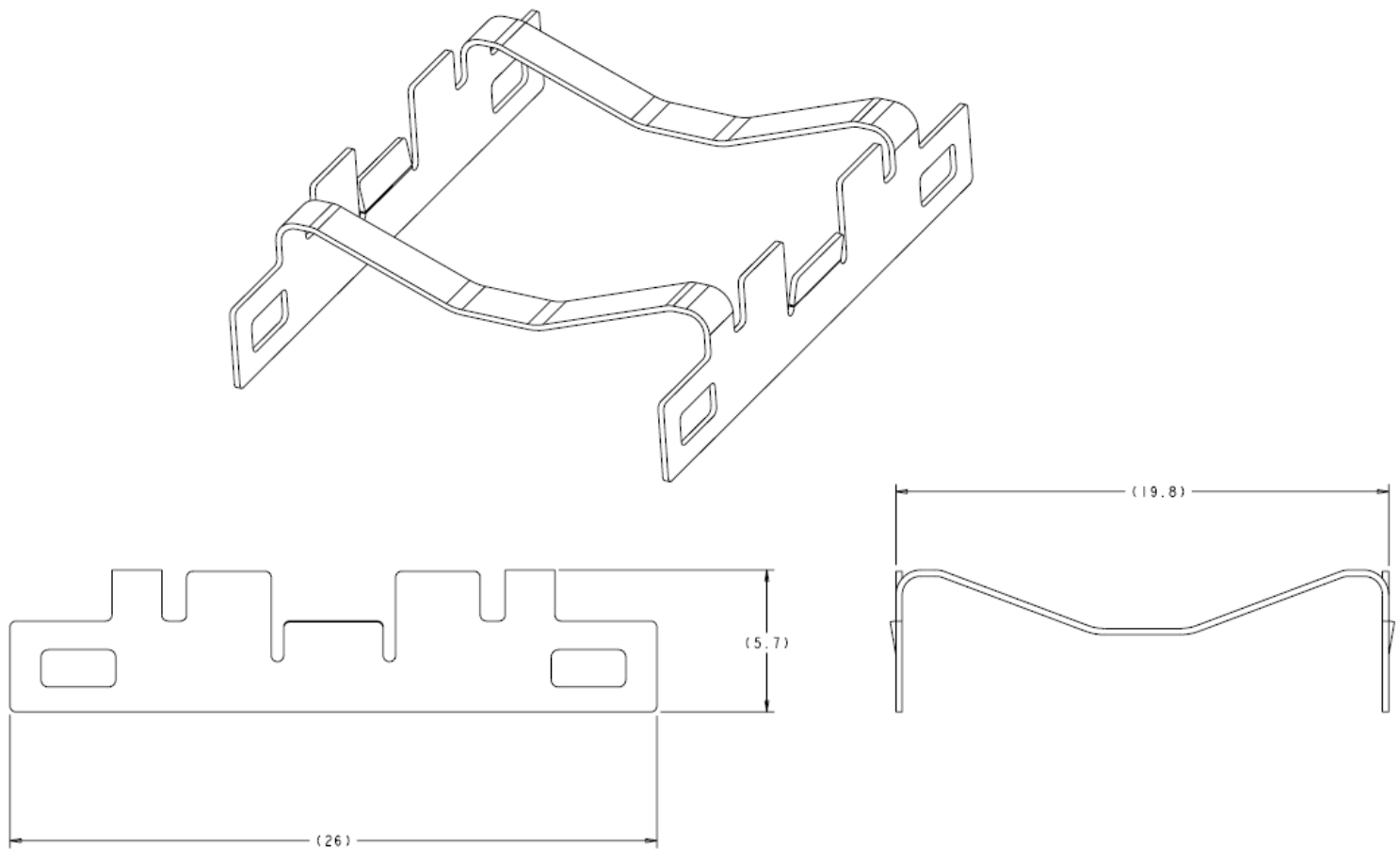
Figure 18 — QSFP+ Heat Sink Clip
