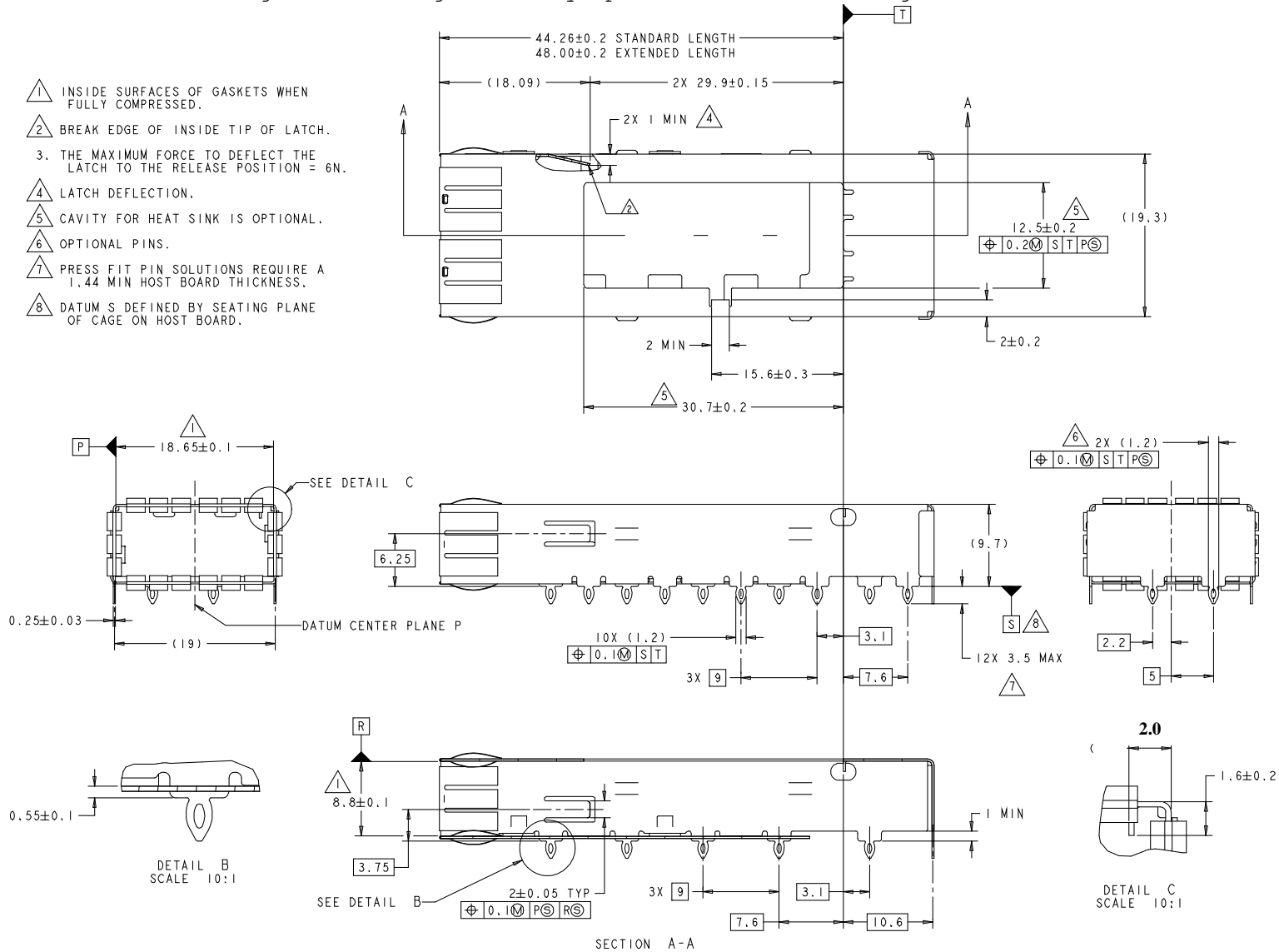
Figure 17A — 1-by-1 Thru Bezel Cage Design
