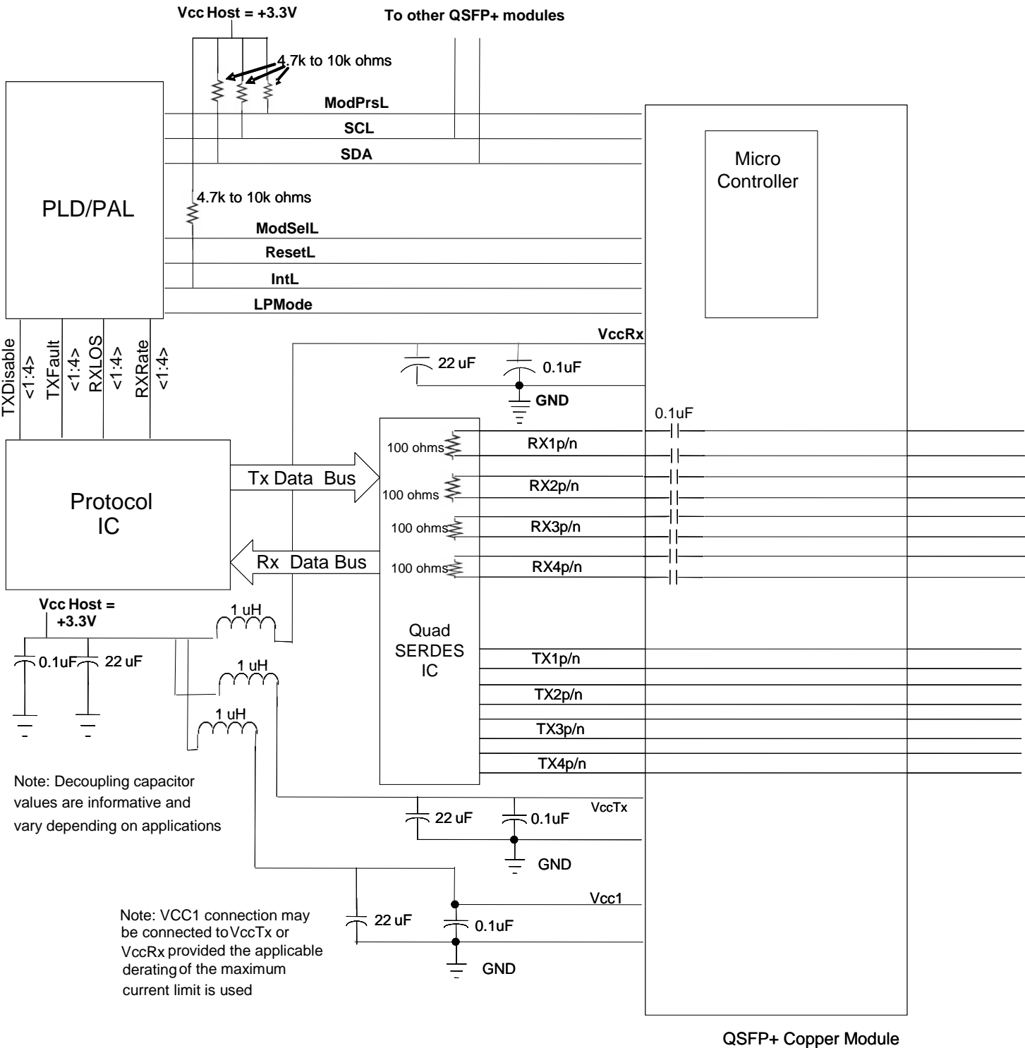
1 2 3 4 Figure 3b Example QSFP+ Host Board Schematic for passive copper cables
