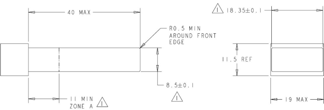
6 7 8 9 Figure 20 — Dust / EMI Cover
