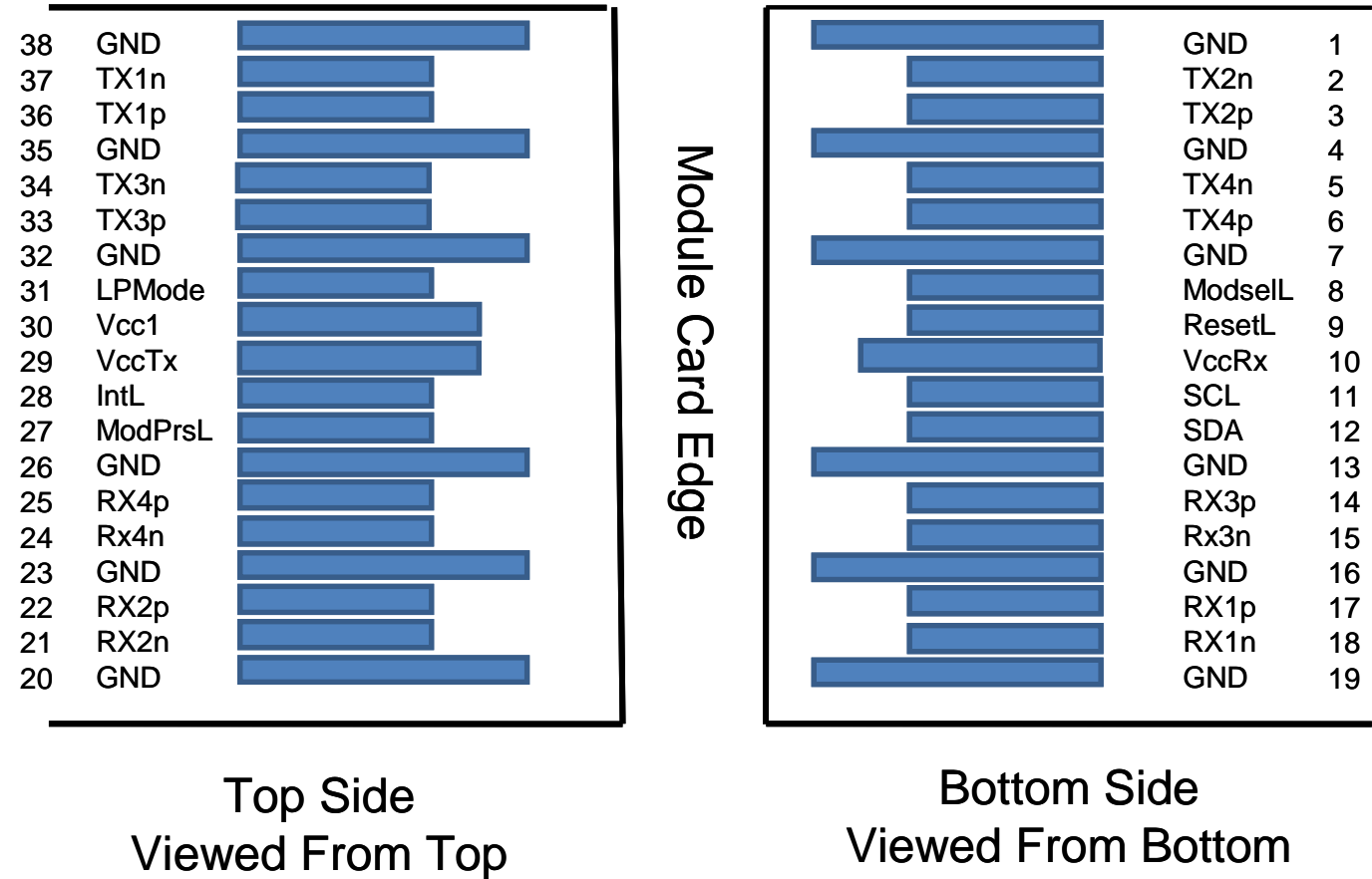
Figure 2 QSFP+ Module Pad Layout
