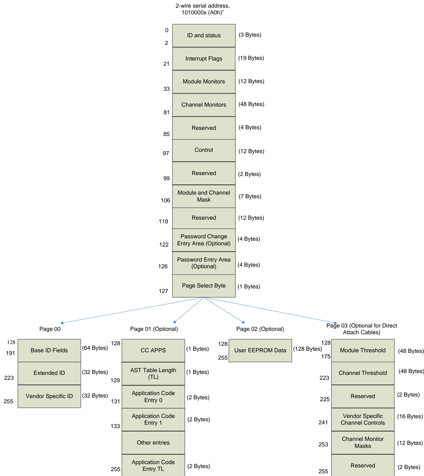
Figure 30 — QSFP+ Memory Map
