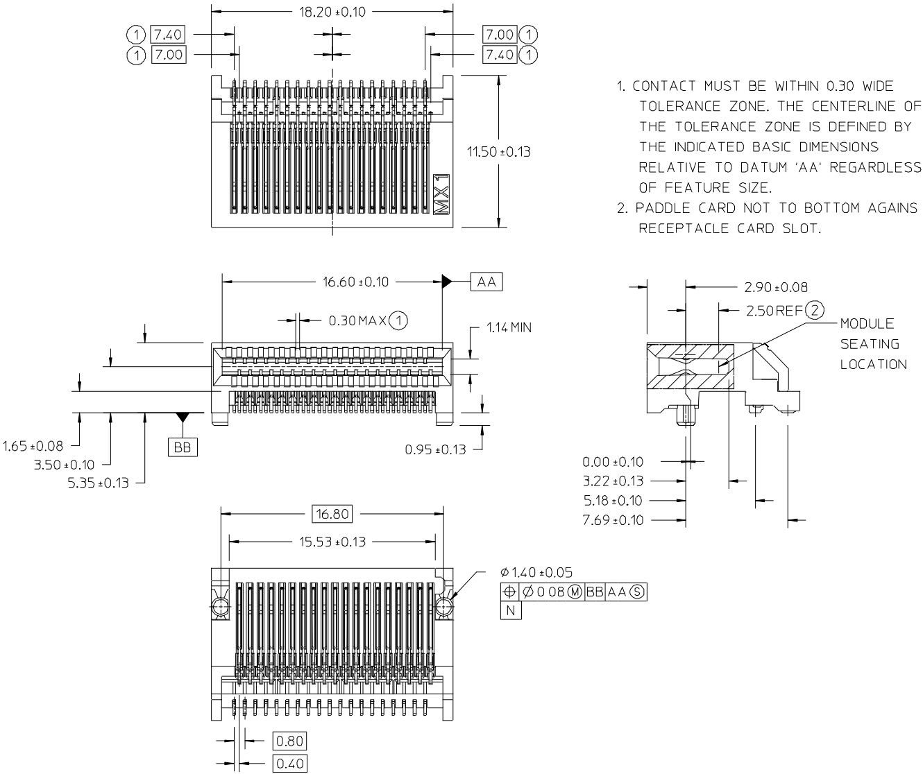
Figure 15 — QSFP+ Electrical Connector Specification
